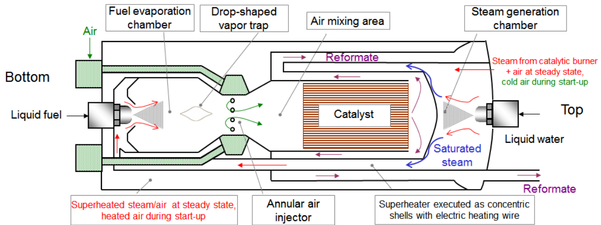
Figure 2 Design of Jülich's autothermal reformer, ATR 14
