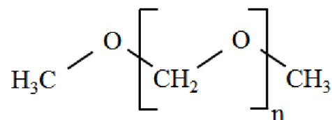
Figure 1 Structural formula of polyoxymethylendimethylether
